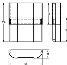
HOUSING EXTENSION FOR SHOWER PANEL
