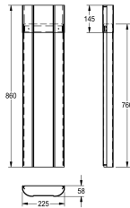
HOUSING EXTENSION FOR SHOWER PANEL
