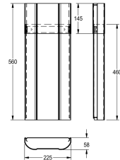
HOUSING EXTENSION FOR SHOWER PANEL
