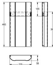
HOUSING EXTENSION FOR SHOWER PANEL
