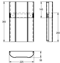
HOUSING EXTENSION FOR SHOWER PANEL
