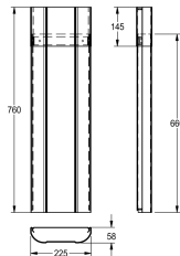
HOUSING EXTENSION FOR SHOWER PANEL
